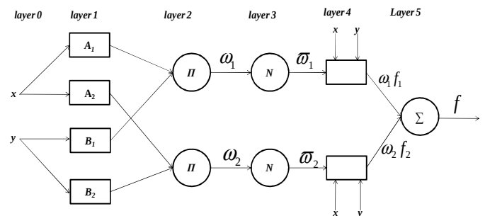
Fig.9: ANFIS architecture
